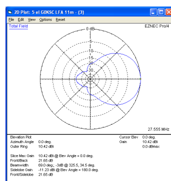
Elevation Plot
