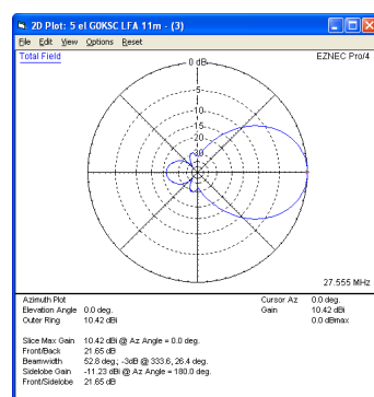
Azimuth Plot
