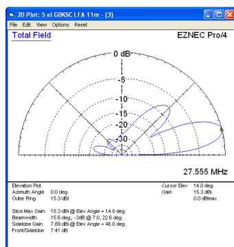
Single 5 element LFA up 10m above ground
