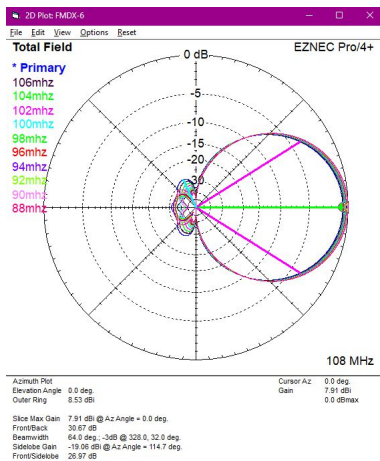
88-108MHz performance plot over-lays showing the impressively consistant performance of the FMDX6
