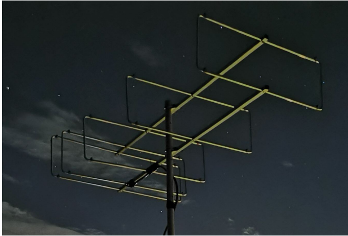
A 5 element High Gain, Super-small 144MHz LFA-Q Quad style Yagi
