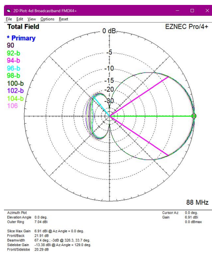
88-108MHz performance plot over-lays showing the impressively constant performance of the FMDX4+
