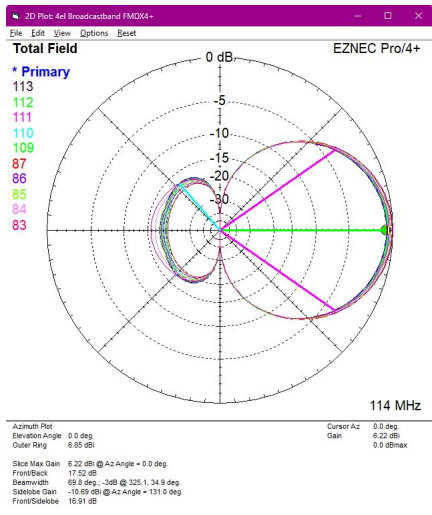
Plot overlay showing out of band coverage (83-87MHz, 109-114MHz) with equally impressive results
