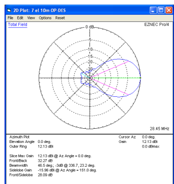
Azimuth Plot at 28.45MHz
