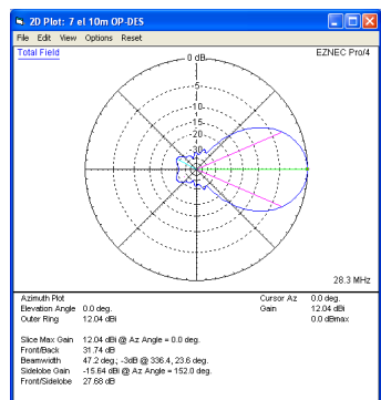
Azimuth plot at 28.3MHz
