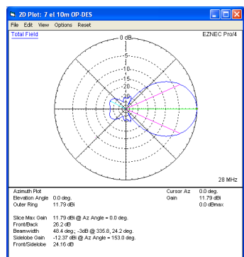
Azimuth plot at 28.0MHz
