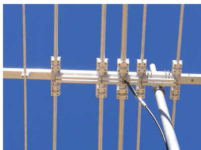
Close-up of the feed arrangement on the XR7 with straight, parallel lines
