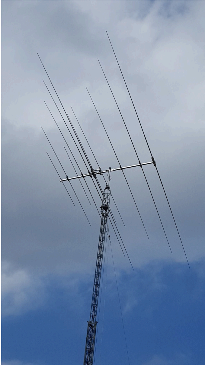
Best HF Yagi Antenna - XR6 MKII - 11 element 6 band HF & 6m Yagi (20/17/15/12/10/6) with 3.5m boom - The World's shortest 6 band HF & 6m Yagi 'full sized' Yagi - InnovAntennas
