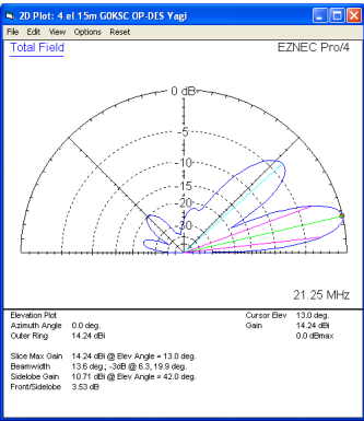
Single 4 element OP-DES up 15m above ground
