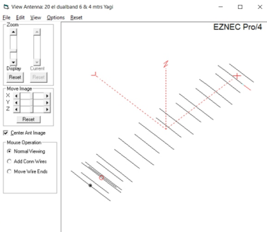
The 4-6-20 element layout
