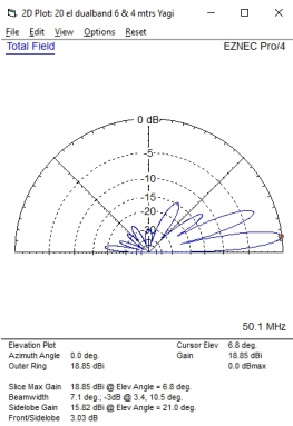
Elevation Plot 50MHz (12m above ground including ground gain)
